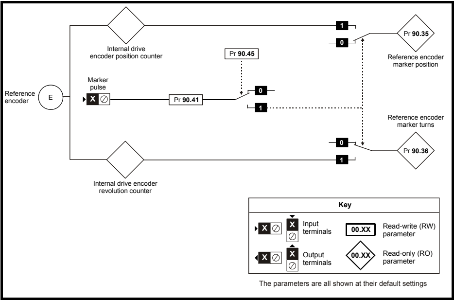
Figure 8-5 Second Processor Reference Marker
