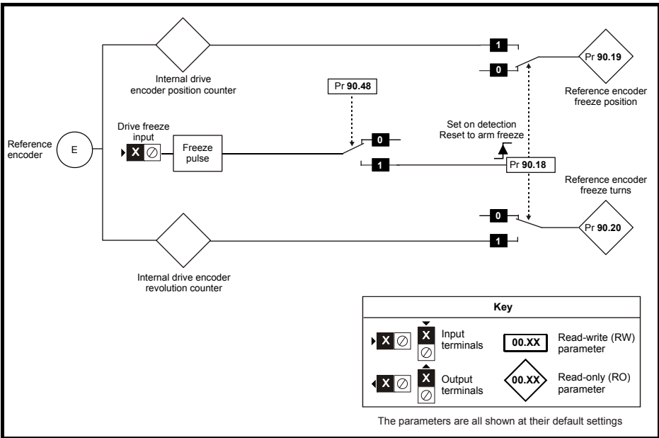
Figure 8-4 SI-Applications Lite V2 Feedback Freeze Input
