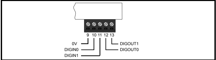
Figure 3-8 Digital I/O Connections
