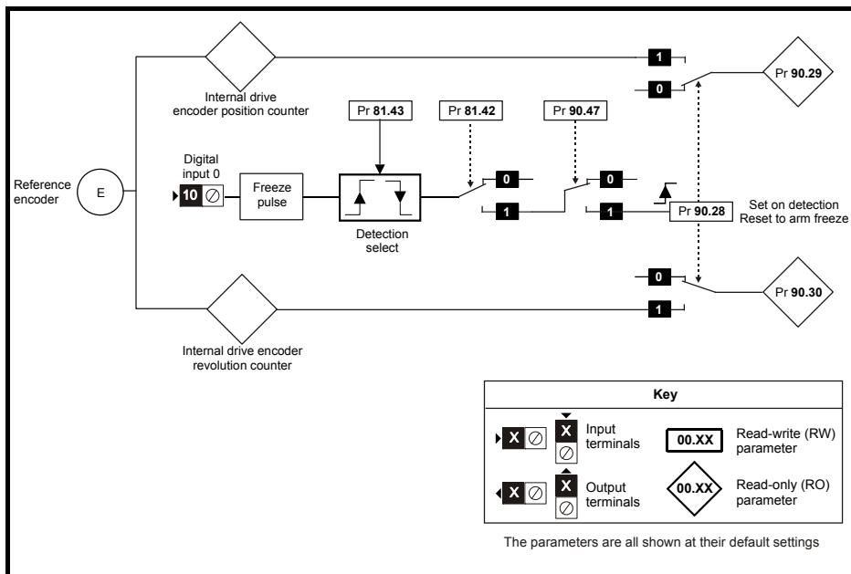
Figure 8-1 SI-Applications Plus and SI-Register Reference Freeze Input
