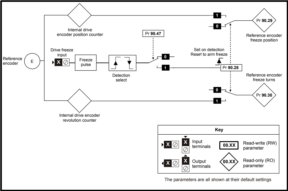
Figure 8-3 SI-Applications Lite V2 Reference Freeze Input
