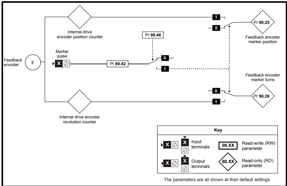
Figure 8-6 Second Processor Feedback Marker
