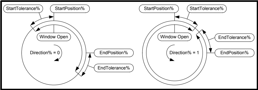
Figure 10-10 Registration window setup
