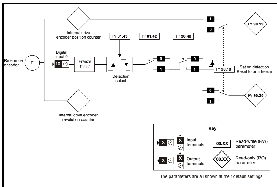
Figure 8-2 SI-Applications Plus and SI-Register Feedback Freeze Input
