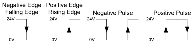
Figure 10-5 Pulse and edge definitions
